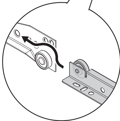
Drawer Slide Under Cabinet Slide
